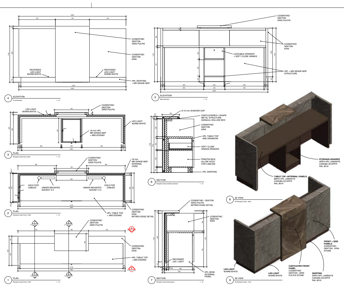
Joinery details
